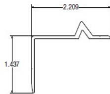
Sill Plate w/ Water Dam
