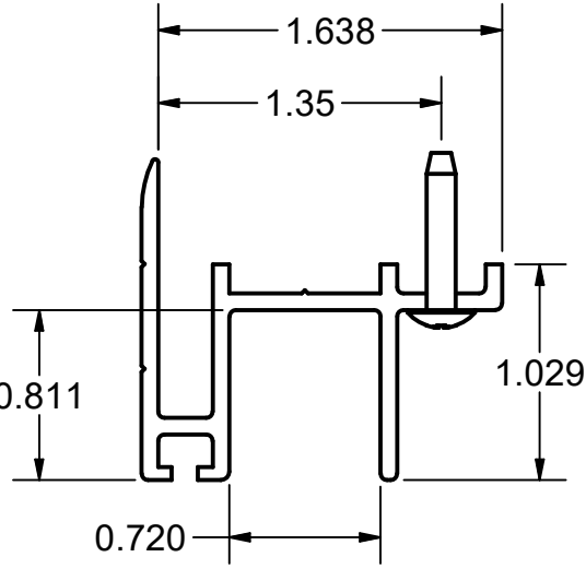
R03975 CONVENTIONAL TRACK (STANDARD)
