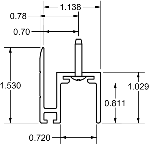
R03976 RECESSED TRACK
