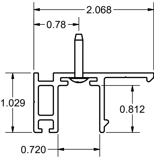
R03730 INTERIOR INTEGRATED TRACK
