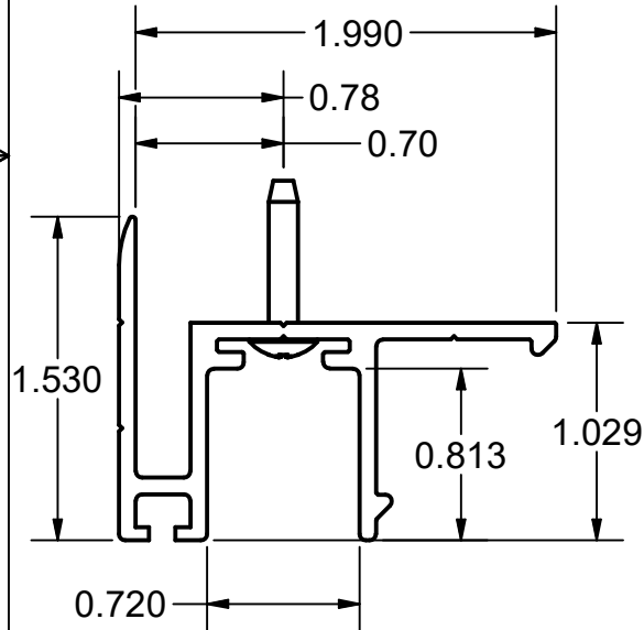
R03977 INTEGRATED TRACK
