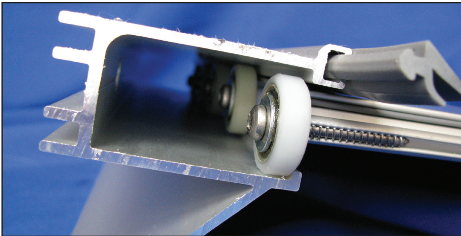
This cut away view illustrates the 1¼" of play inside the track system that reduces the cover from binding. Urethane wheels and stainless steel bearings and hardware ensure long life
